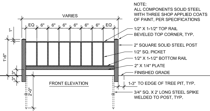
TREE PIT GUARD TYPE 'K' NOT TO SCALE
