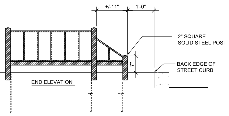
TYPE 'K' THREE-SIDED DESIGN NOT TO SCALE
